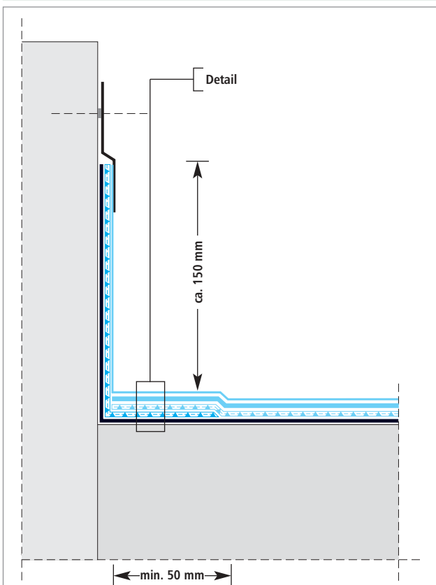
Upstand with cover flashing
