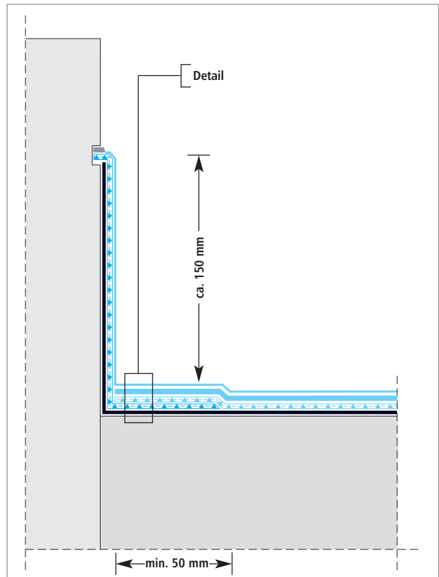
Upstand with chase
