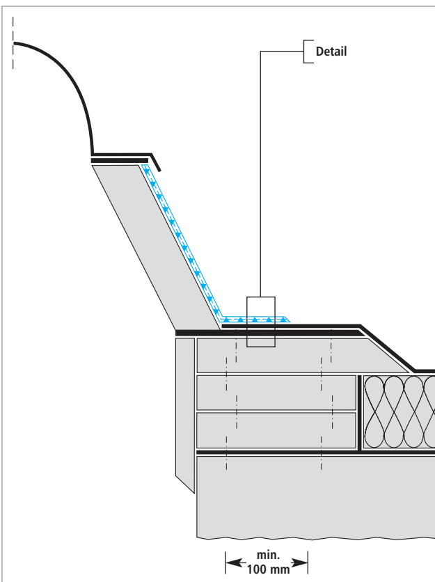
Rooflight
