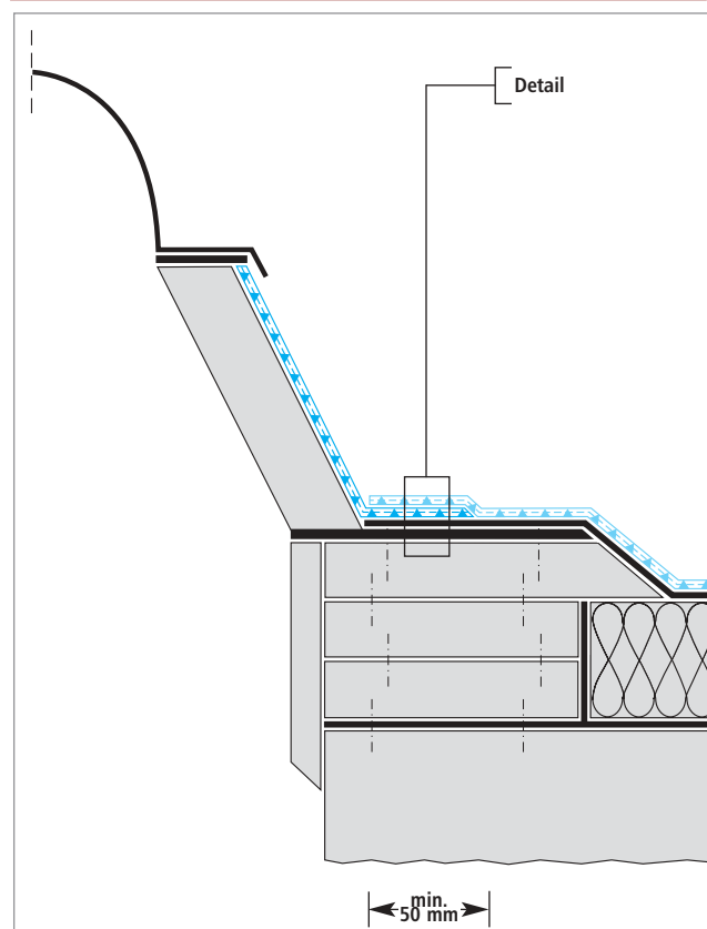
Rooflight
