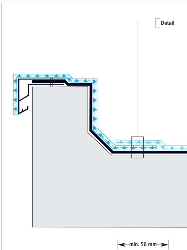
Check kerb to roof edge
