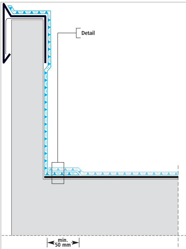
Parapet over capping
