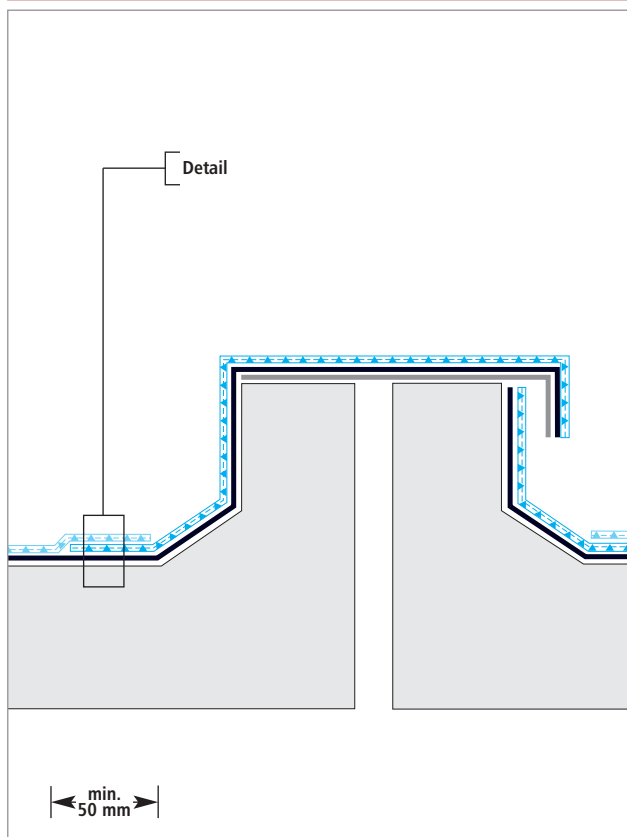
Twin kerb expansion joint
