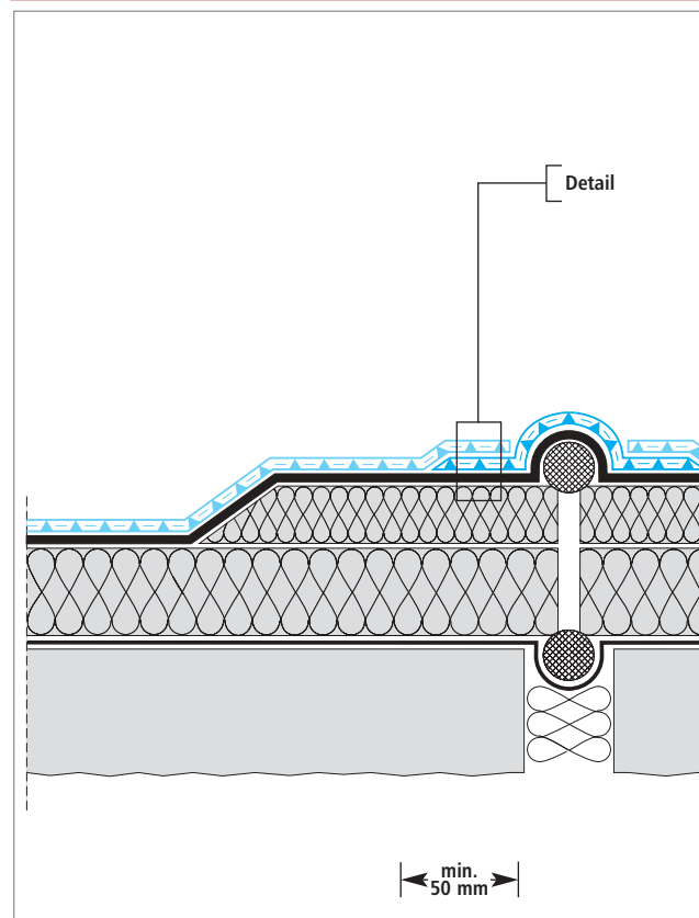
Raised expansion joint
