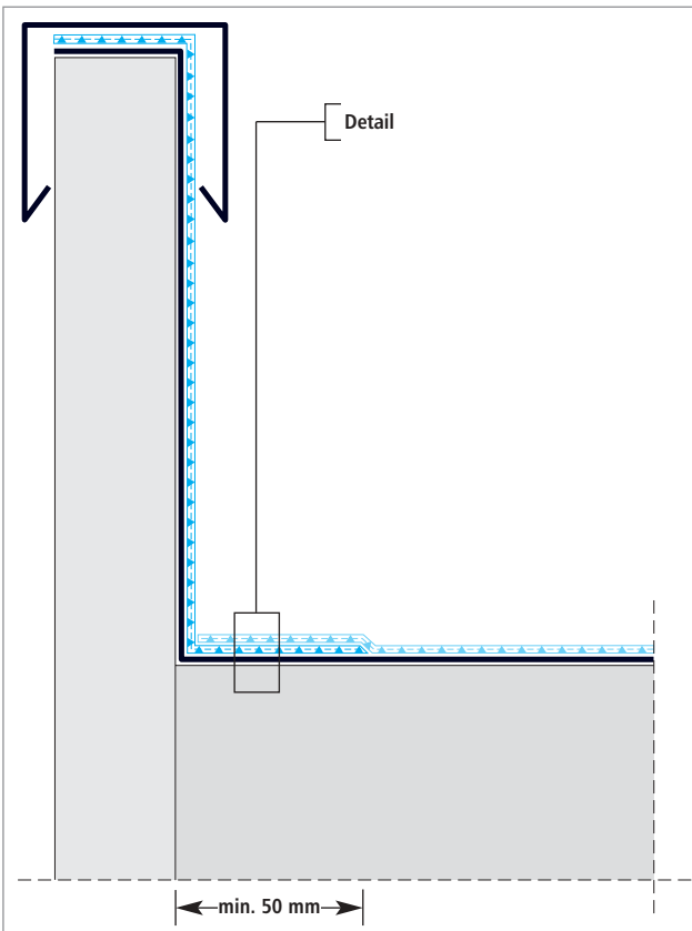
Parapet with capping
