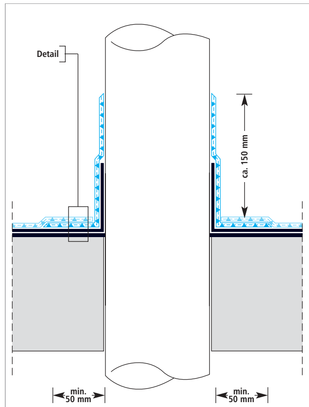
Roof penetration
