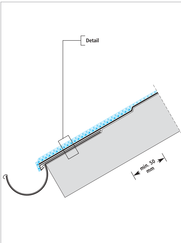
Drip to external gutter
