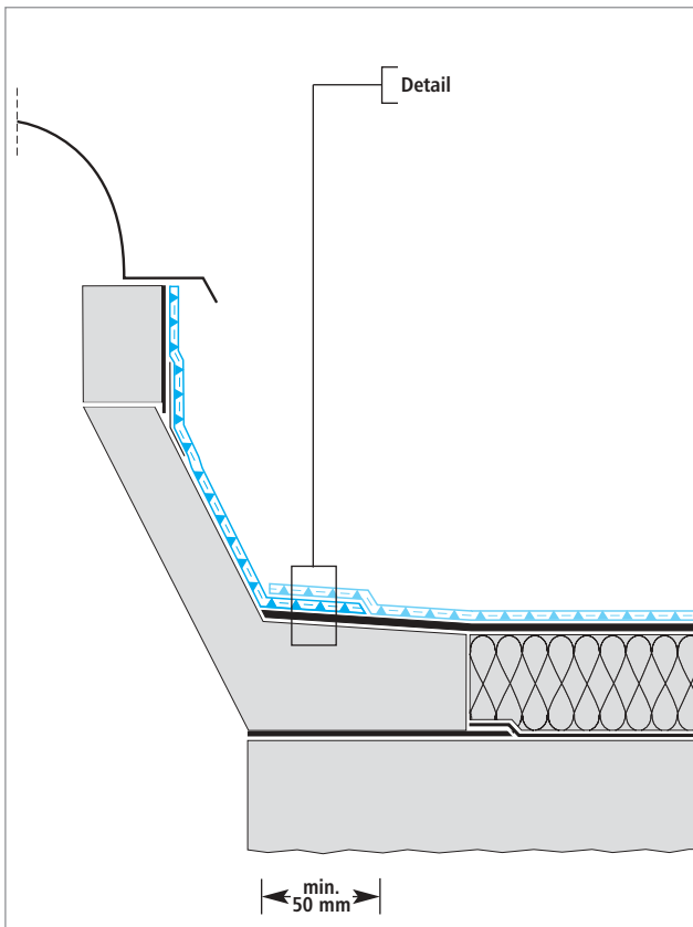
Rooflight with upstand
