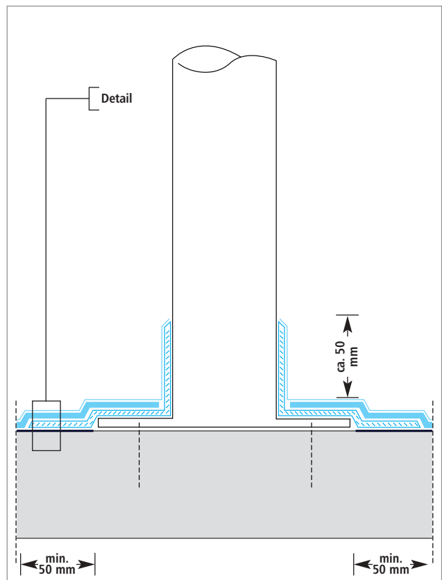
Surface mounted detail - Less Critical
