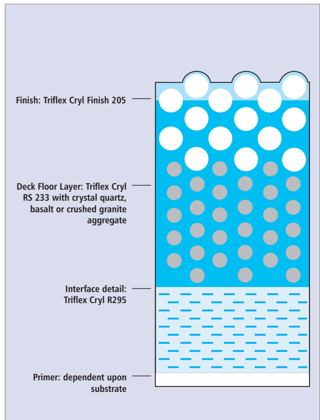
Detail interface - Less Critical
