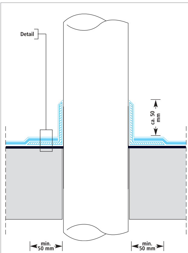
Deck penetration - Less Critical
